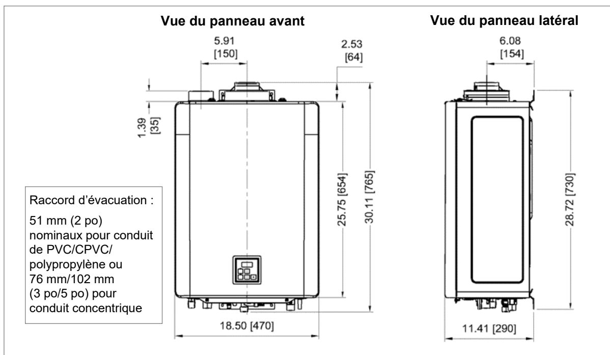
Figure 2 : Dimensions
