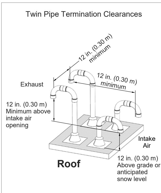
Figure 20: Twin Pipe Vertical Termination of Multiple Water Heaters
