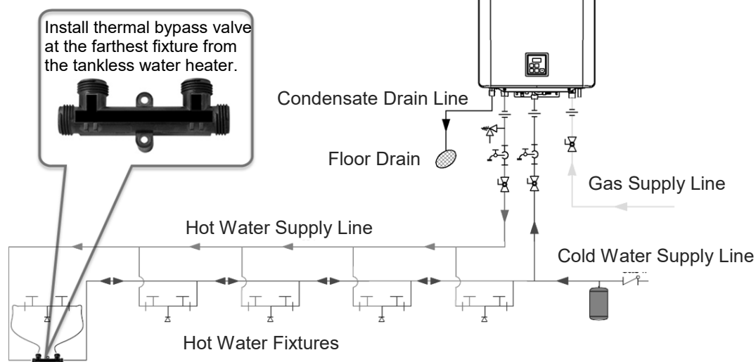
Figure 70: Dedicated Mode
