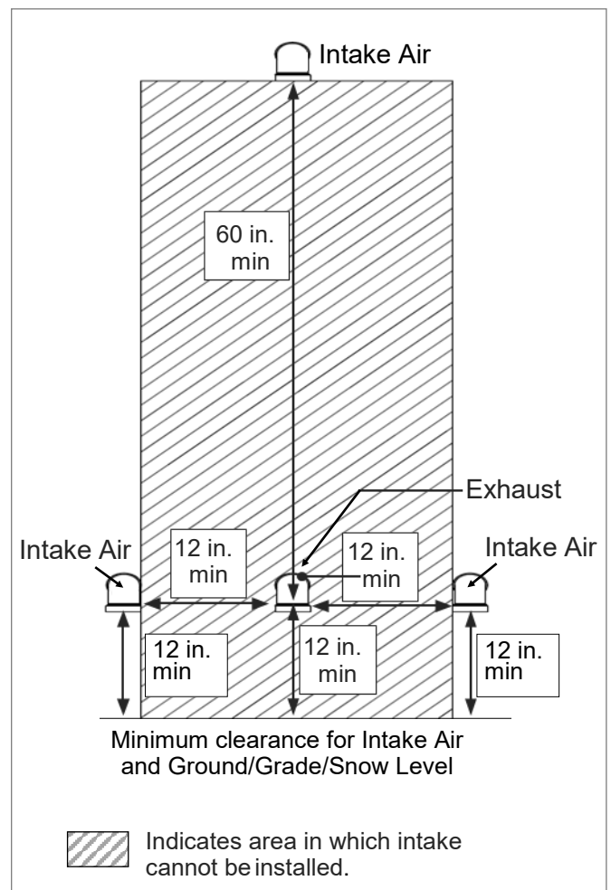
Figure 21: Horizontal Vent and Intake Air Piping
