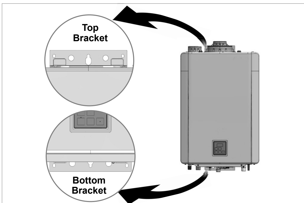
Figure 7: Top and Bottom Bracket
