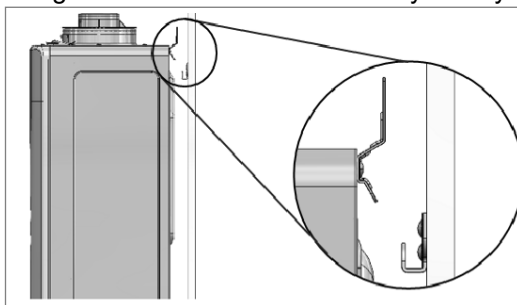
Figure 6: Mount the top bracket
