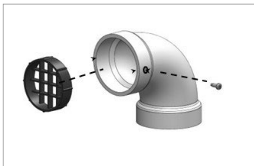
Figure 8: Vent Screen
