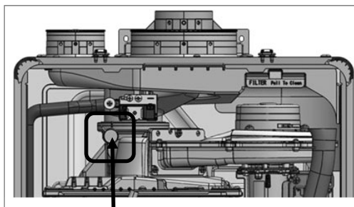
Insert gas analyzer probe into combustion analysis port.
