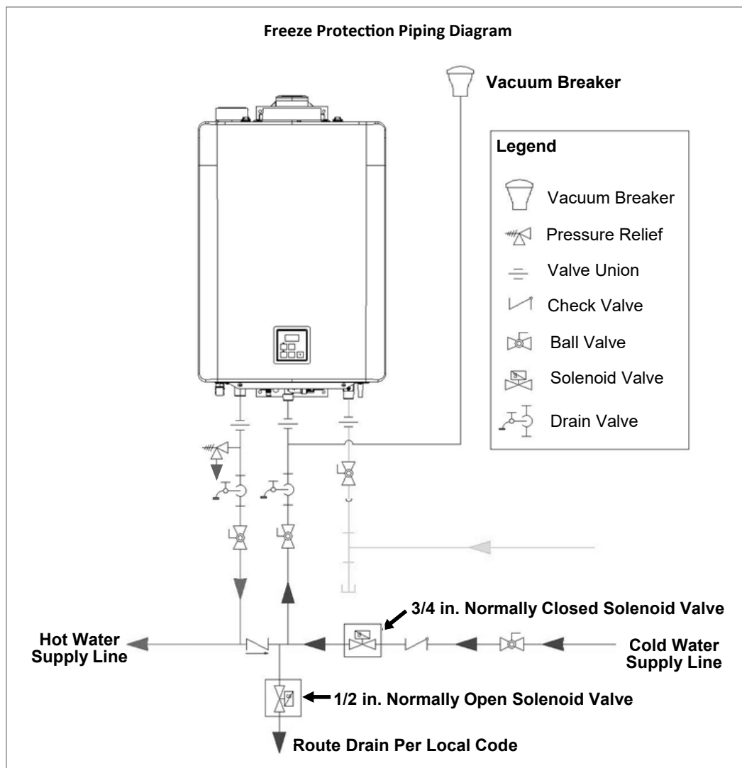
Figure 4: Freeze Protection Piping Diagram
