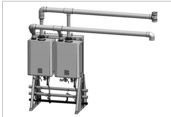
Figure 37: Sample Inline, Freestanding Configuration
