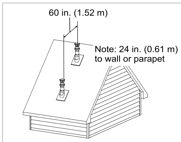
Figure 12: Between terminals at different levels
