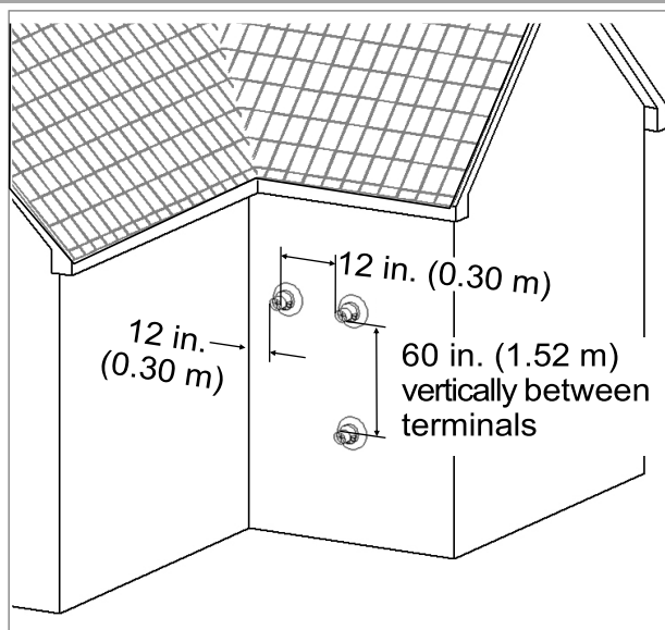
Figure 11: Concentric Pipe Termination Clearances
