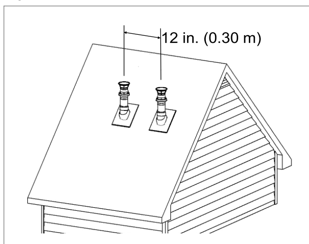
Figure 13: Between terminals at same level
