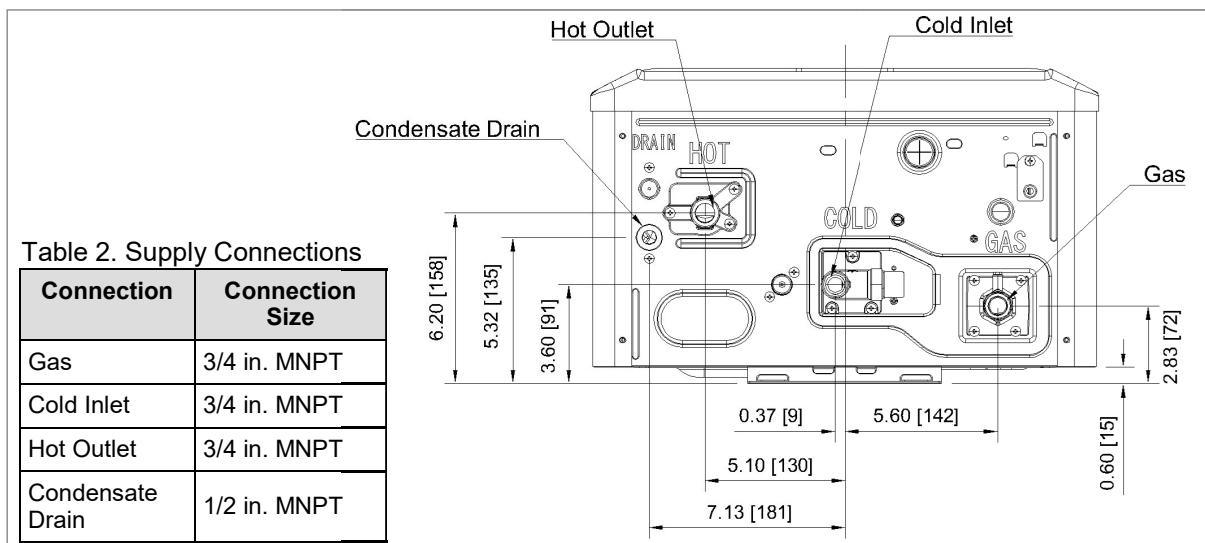
Figure 3: Supply Connections
