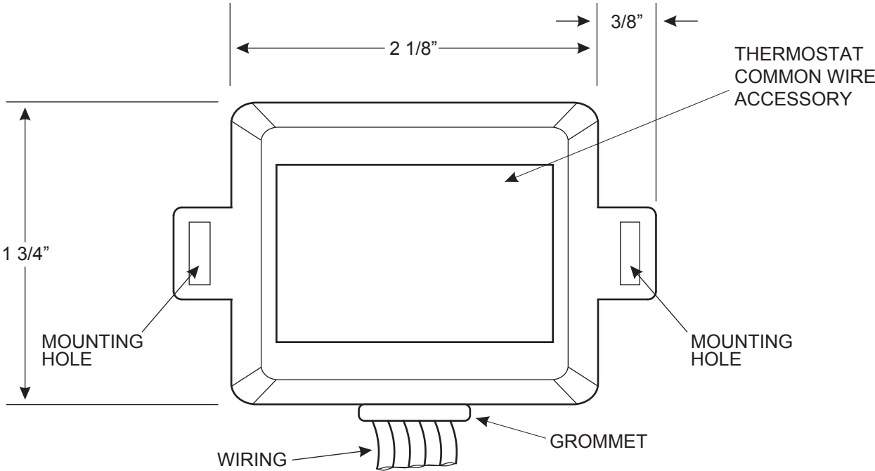
Fig.1 - Thermostat Common Wire Kit Mounting
