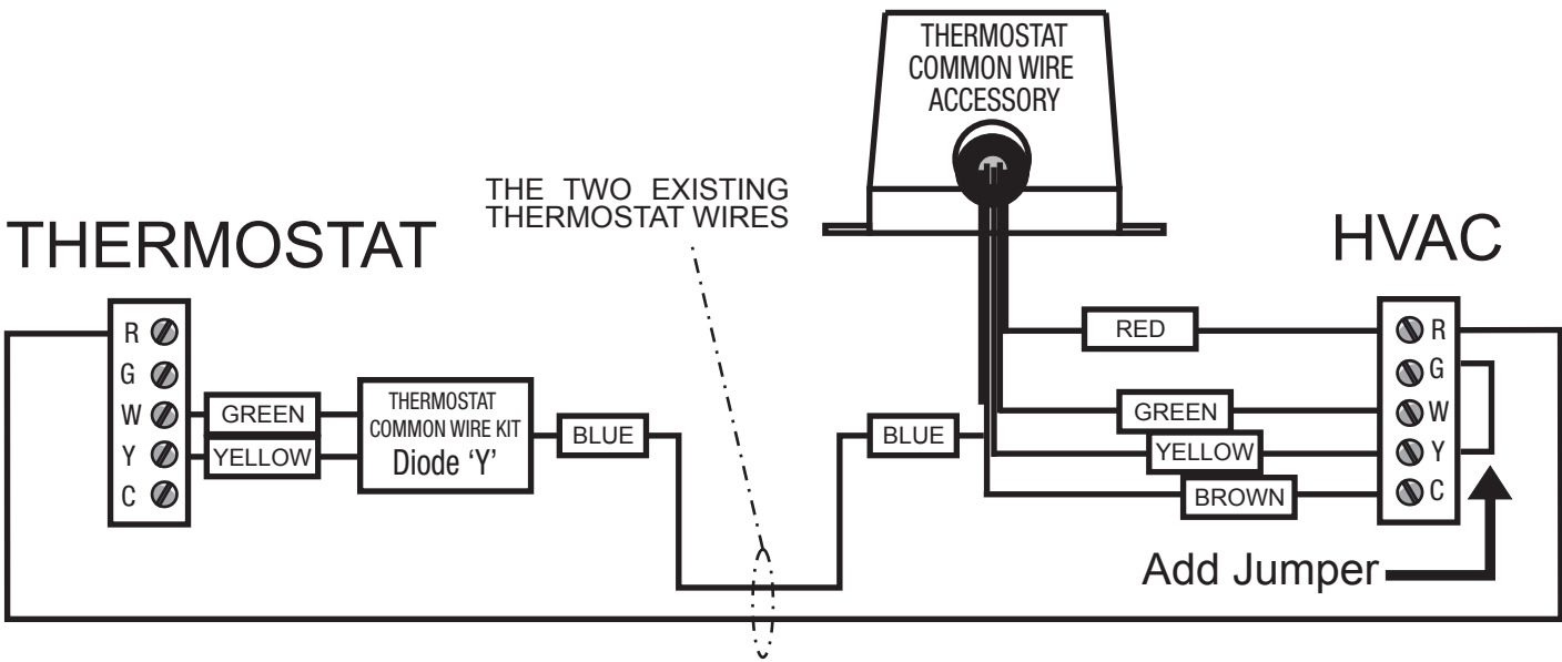
2 existing wires with Thermostat Common Wire Kit to accommodate heating and cooling. No independent fan switching. A jumper is required across G & Y.
